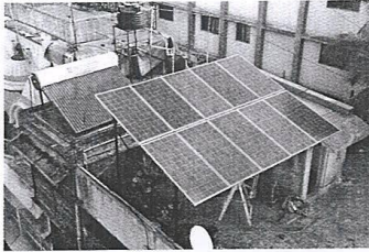
3 KWp elevated roof
