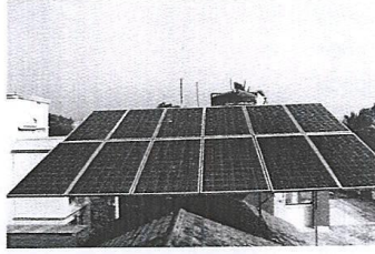
3.6 KWp elevated roof
