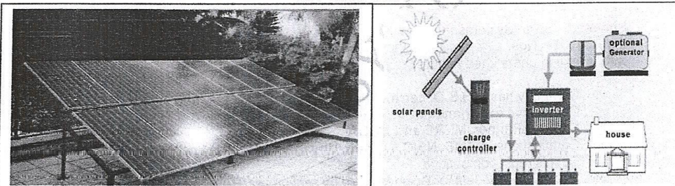
Solar Power Pack Installed by Suryatech Solar Systems, Pune
